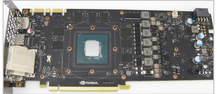
9. Clean the thermal paste from the GPU core and remove any residue left from the thermal pads.
