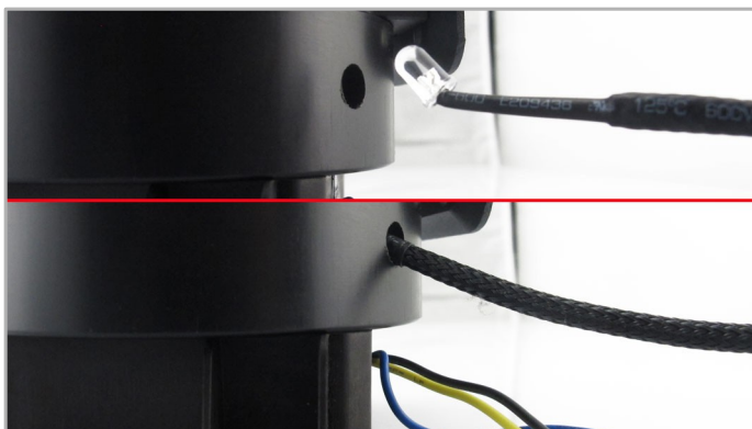
5. Slightly kink the LED wire and push the LED into the hole on the base of the reservoir. You might need to twist the LED slightly until it slots into place.
